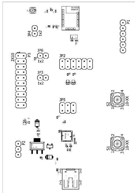
Figure 16: Assembly diagram
