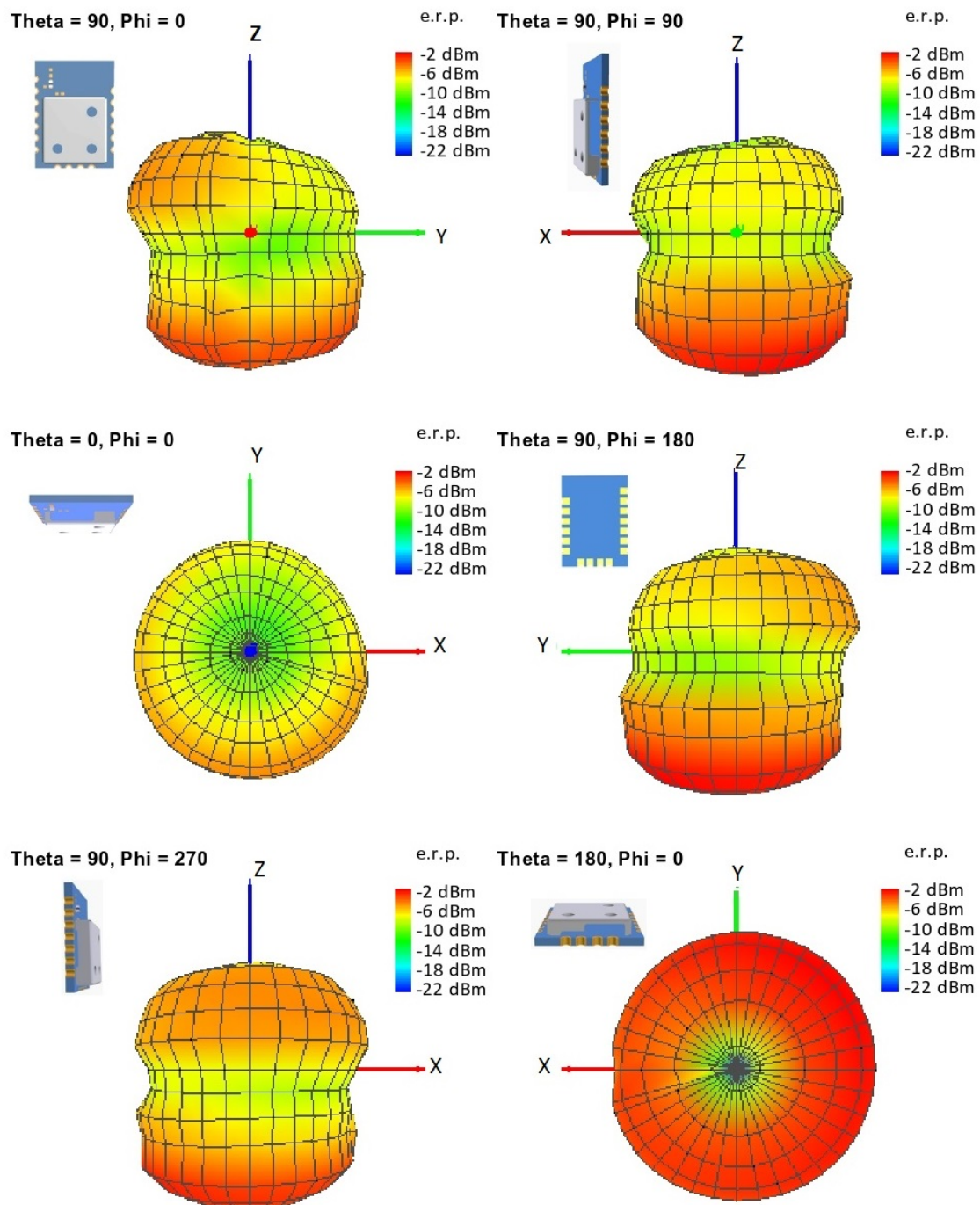
Figure 18: Antenna characteristic from integrated antenna measured on official evaluation board*
