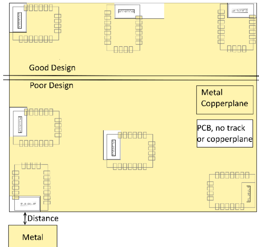
Figure 12: Placement of the module with integrated antenna
